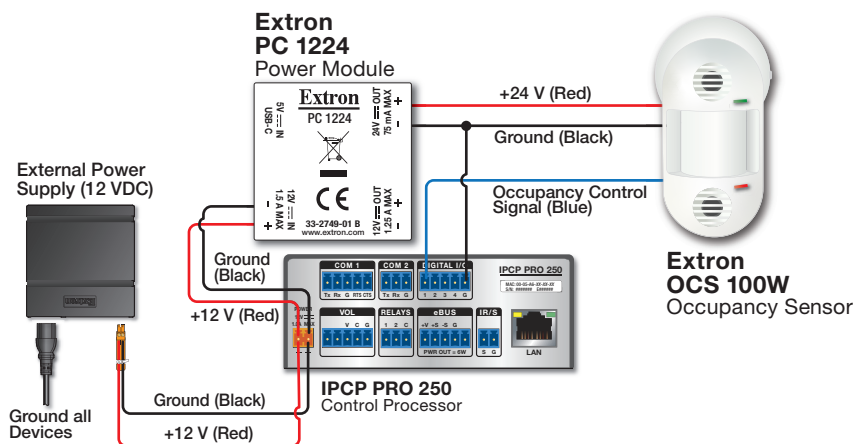
Figure 8. OCS 100W External Power Supply Wiring Diagram
